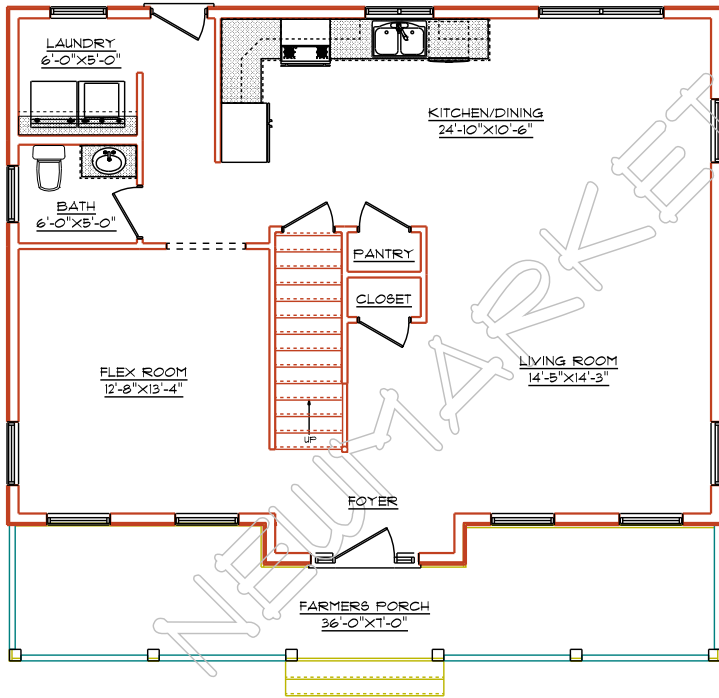
LEVEL ONE PLAN
